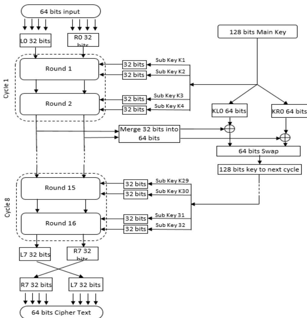
Fig.2 Block diagram ETSET
