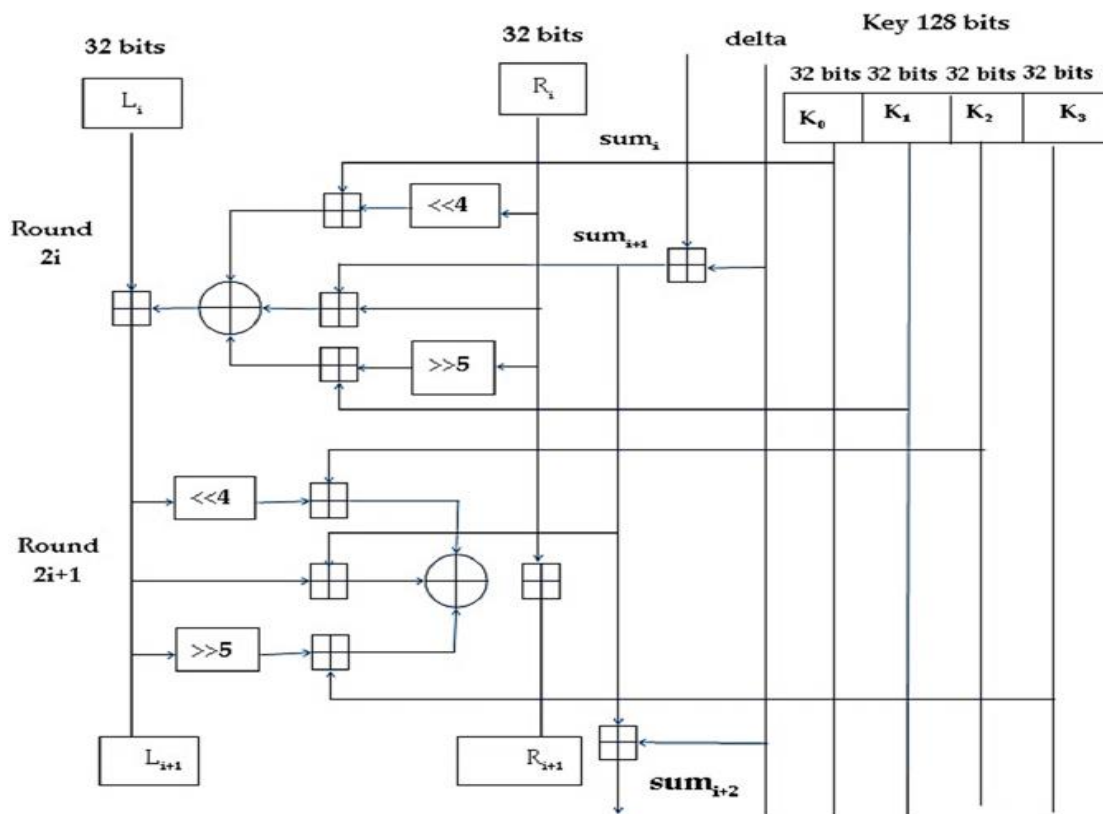
Fig. 1 Block diagram of TEA
